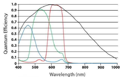
MV-CA050-10GM/GC 量子效率
